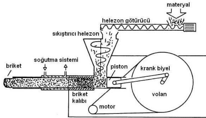
Şekil 1.3. Piston presli briketleme makinesi (Werther vd, 2000; Karaca, 2009)
